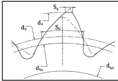
FIG. 7: ASYMMETRIC TOOTH PARAMETERS
