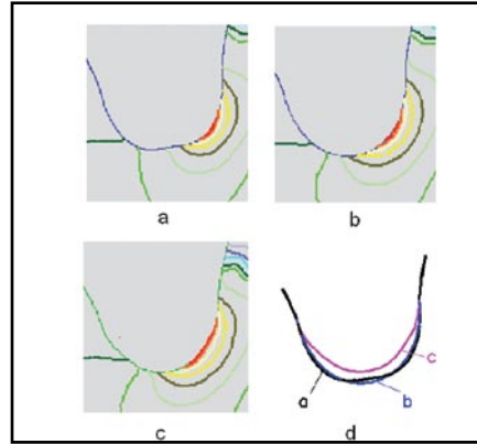
FIG 3: BENDING STRESS DISTRIBUTION ALONG THE FILLET; A—THE STANDARD AGMA 201.02 20 DEGREE RACK GENERATED FILLET; B—THE FULL RADIUS 20 DEGREE RACK GENERATED FILLET; C—THE OPTIMIZED FILLET; D - THREE FILLET OVERLAY.
