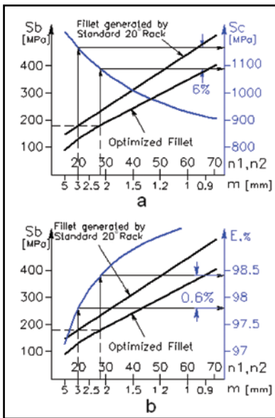
FIG. 4: A—CONTACT STRESS REDUCTION; B—INCREASED MESH EFFICIENCY.
