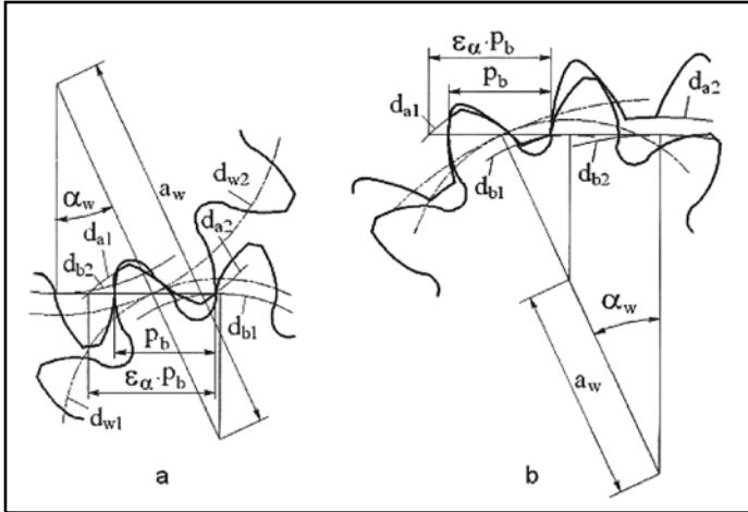
FIG 2: GEAR MESH; a—EXTERNAL GEARING; b—INTERNAL GEARING; a_w —CENTER DISTANCE; p_b —BASE CIRCLE PITCH; \alpha_w —OPERATING PRESSURE ANGLE; \epsilon_\alpha \cdot p_b —CONTACT RATIO; d_{w1,2} —OPERATING PITCH CIRCLE DIAMETERS; SUBSCRIPTS “1” AND “2” ARE FOR THE MATING PINION AND THE GEAR.
