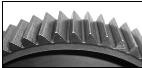
FIG. 6: GEAR WITH ASYMMETRIC TEETH
