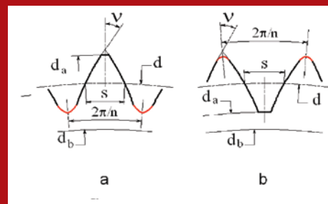
FIG 1: TOOTH PROFILE (THE FILLET PORTION IS RED); A—EXTERNAL TOOTH; B—INTERNAL TOOTH; d_a —TOOTH TIP CIRCLE DIAMETER; d_b —BASE CIRCLE DIAMETER; d —REFERENCE CIRCLE DIAMETER; s —CIRCULAR TOOTH THICKNESS AT THE REFERENCE DIAMETER; \nu —INVOLUTE INTERSECTION PROFILE ANGLE.
