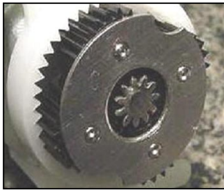
FIG. 11: THE PLANETARY DRIVE FOR AN AUTOMATION APPLICATION. THE GOAL WAS TO PROVIDE A HIGH GEAR RATIO (63:1) IN ONE PLANETARY STAGE AND HIGH OUTPUT TORQUE IN A VERY LIMITED SPACE. THE GEAR ARRANGEMENT OPTIMIZATION IN COMBINATION WITH DGD PROVIDED SUCCESS IN ACHIEVING THIS GOAL.
