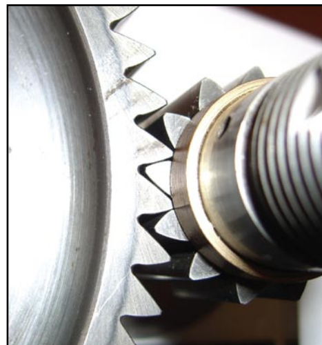
FIG. 14: IN THESE GENERATOR GEARS, APPLICATION OF THE ASYMMETRIC FOR THE EXPERIMENTAL GENERATOR GEAR DRIVE ALLOWED FOR A SIGNIFICANTLY REDUCED VIBRATION LEVEL.
